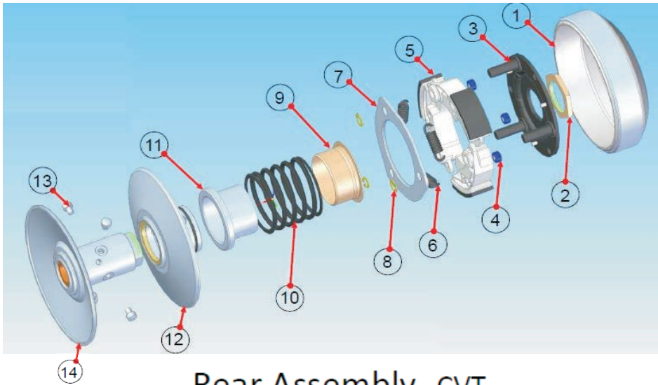
Rear Assembly- CVT
