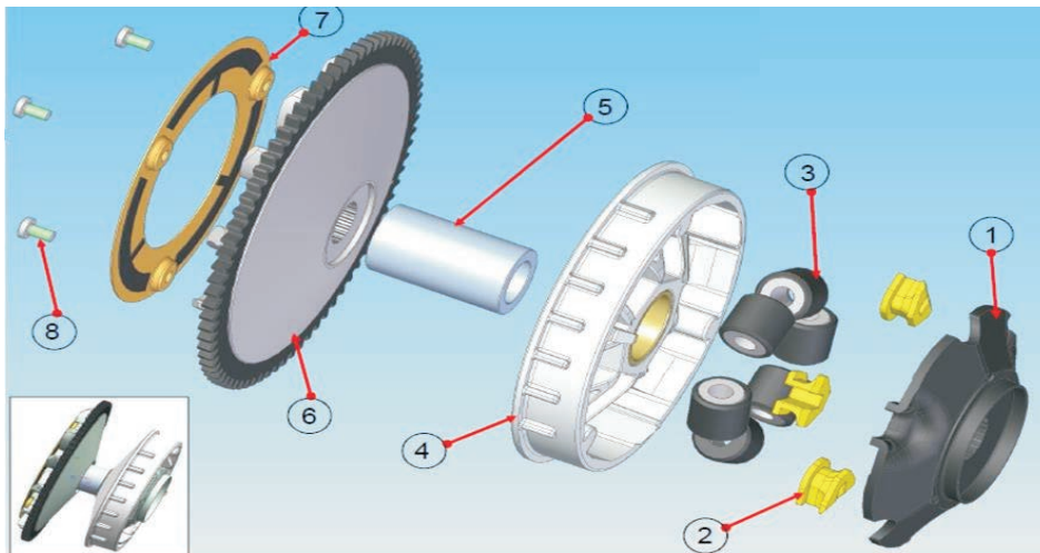
Front Assembly- CVT
